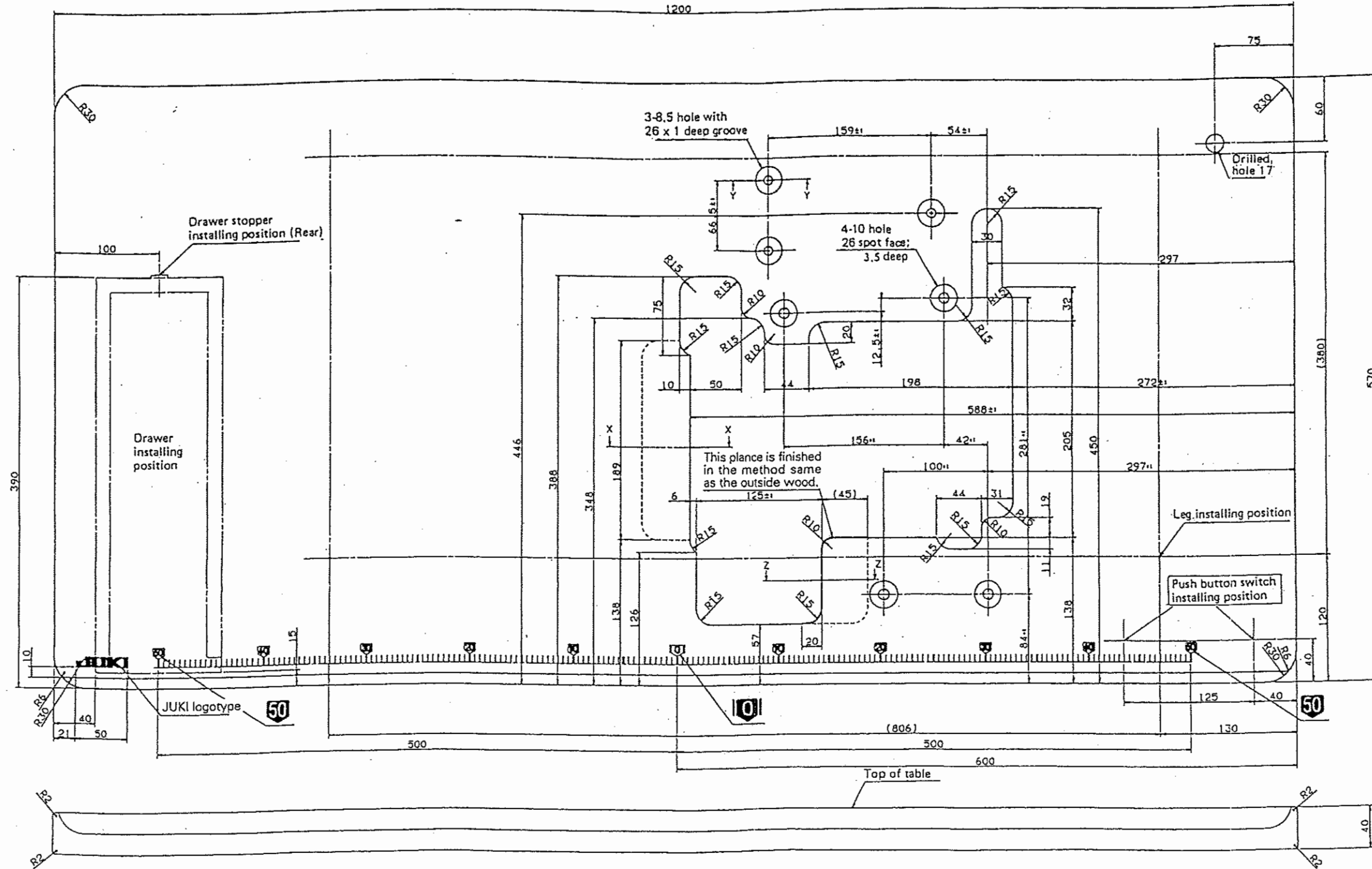
Detailed measurement diagram (2:1)
