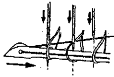
One chain stitch by middle needle
